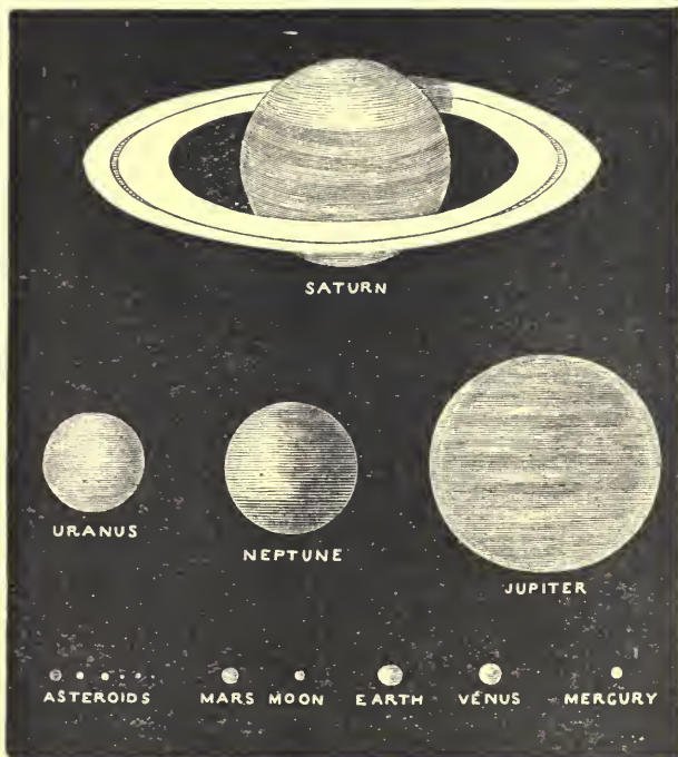
Fig. 5.—Comparative sizes of Planets.
